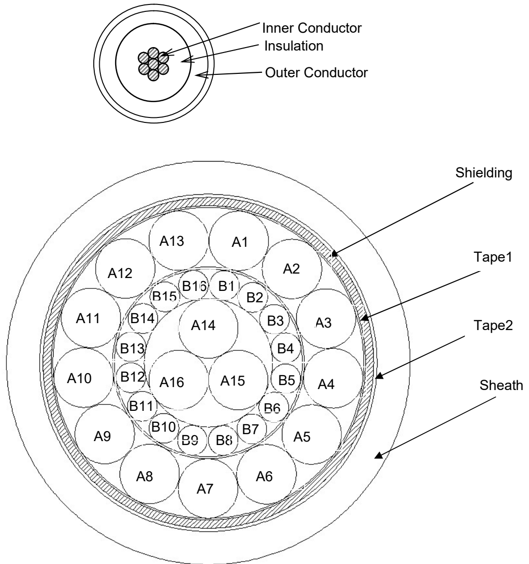
Fig.1 Cross section view of cable
