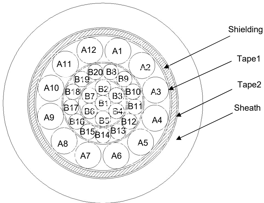
Fig.1 Cross section view of cable
